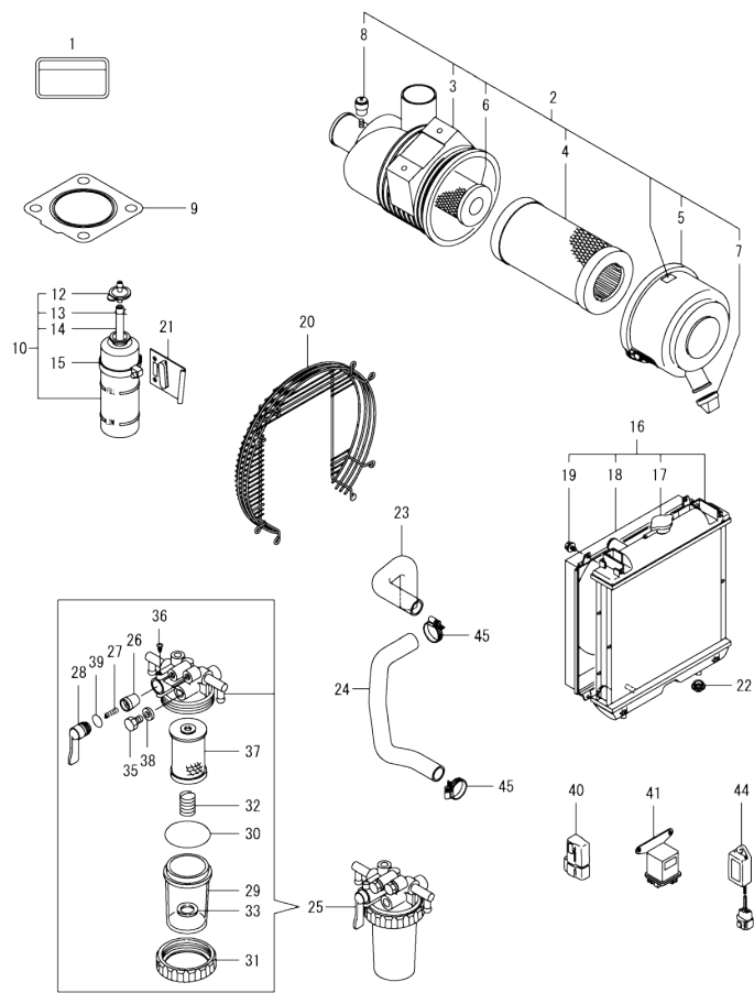
OCD50-M04990 ENGINE Fig.16. ACCESSORY
